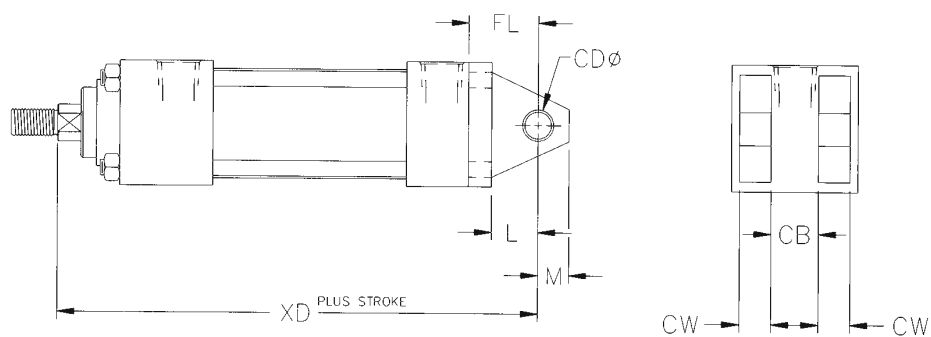
Mount Code P2 NFPA MP2
