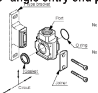
D801-00-(20,25)-W-B81W Distributor Block
