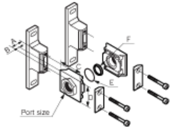
A800-(20,25,32)-W-B81W Straight end Plate Kit
